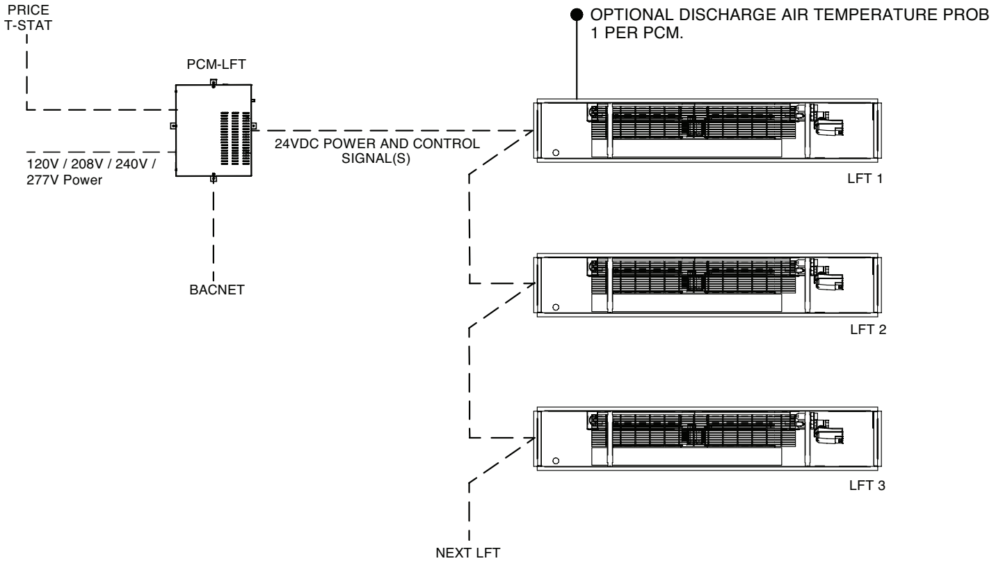
FIGURE 11: LFT WIRING (ACTUATORS BY OTHERS) ▼
