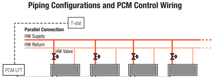
FIGURE 5: LFTs IN PARALLEL CONFIGURATION
