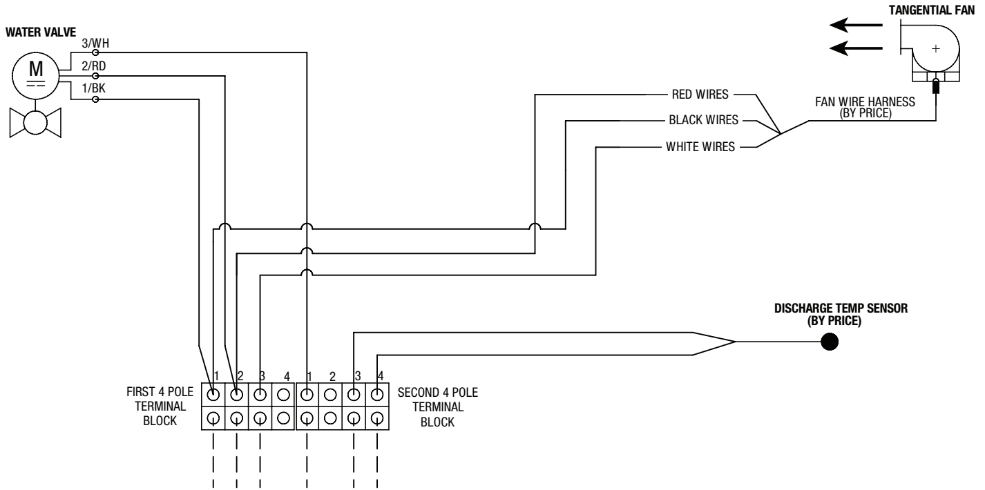
FIGURE 10: LFT TERMINAL BLOCK WIRING ▼
