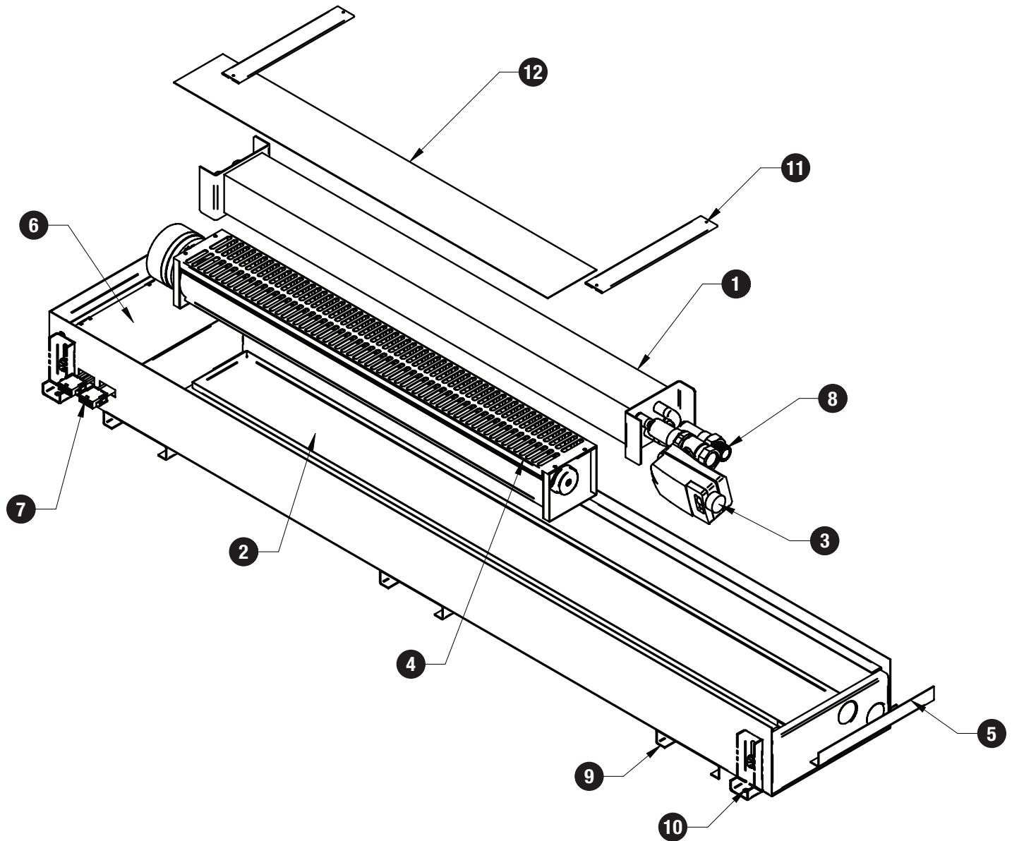
FIGURE 1: LFT - ISOMETRIC “NON - FLANGED BORDER SHOWN” ▼
