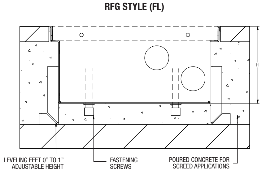
FIGURE 4: LFT FLARED PLENUM SIDE VIEW ▼
